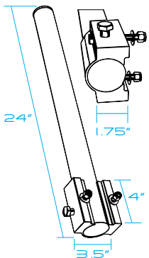
NEW Dock Mount Kit Complete with bolts & Dock Pole Bushing
