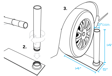
Wheel Stand DP-WS DP-WSJ (for JR poles)
