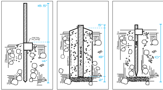
Ground Stakes For temporary install of 13.5', 19' & 22' Telescoping Poles Ground Sleeves For permanent install of 13.5', 19' & 22' Telescoping Poles Ground Sleeves For temporary & permanent install For JR poles only
